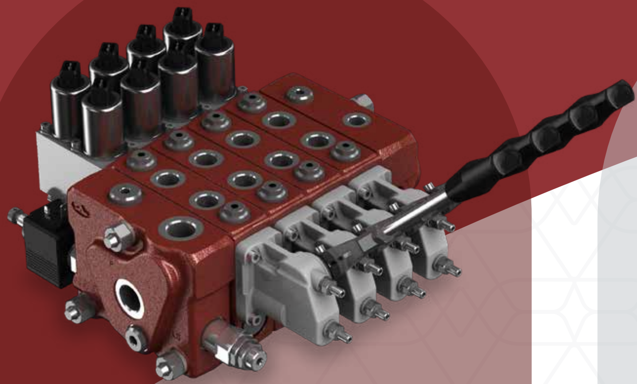
DPX100 Full Flow Sharing directional control valve
